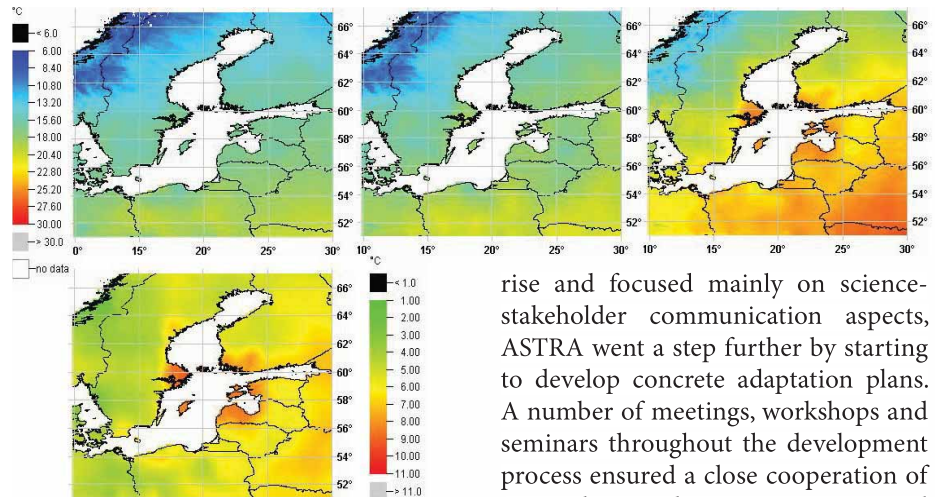
Mean temperature for the summer seasons (June, July, August) for 2001, 2050 and 2099 (upper panel) and the difference 2099/2001 (lower left panel). Source: Potsdam Institute for Climate Impact Research, based on CRU/ATEAM data
